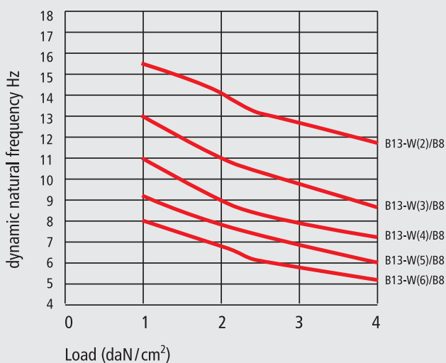
dynamic natural frequency vertical
