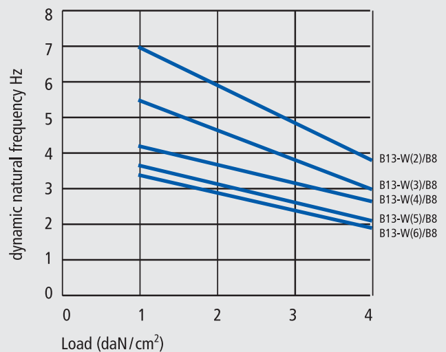
dynamic natural frequency horizontal
